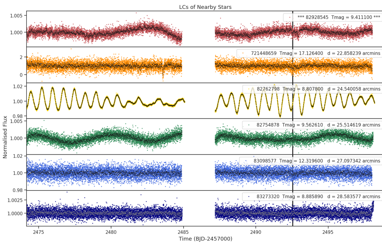
Fig 8. Lightcurves of the five closest stars to target 82928545 (top panel). The distances to the target star and the TESS magnitudes are shown for each star. Only ever shown for one sector.
