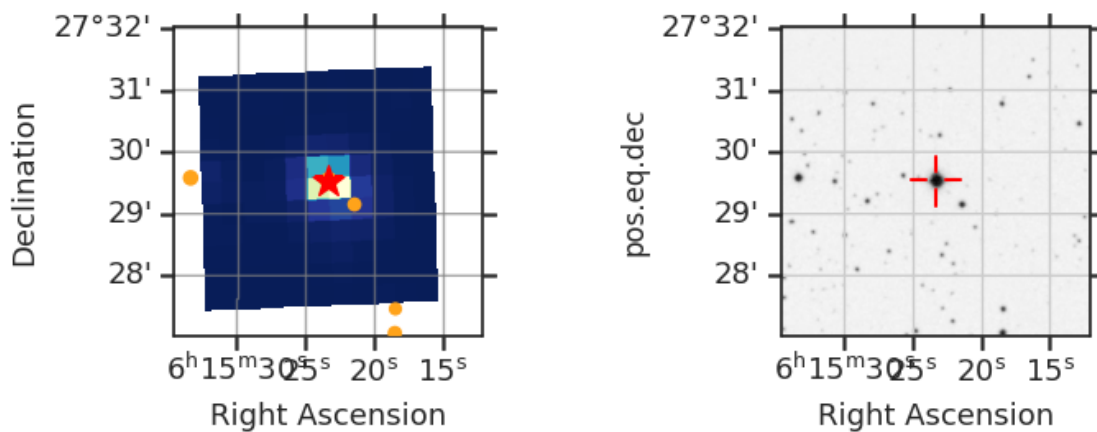
Fig 7. The locations of nearby GAIA DR2 stars with a magnitude difference less than 5 (orange circle) within the Tess Cut Out around TIC 82928545 (red star). Only shown for one sector. Right: SDSS image of the surrounding field.
