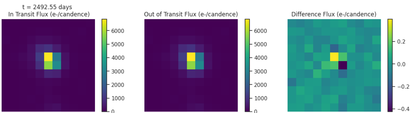
Fig 6. Difference images for target TIC 82928545 for each transit like event. Left: mean in-transit flux(left). Middle: mean out-of-transit flux. Right: difference between the mean out-of-transit and mean in-transit flux. Ensure that the change in brightness occurs on target.
