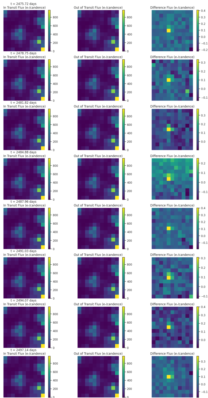
Fig 6. Difference images for target TIC 720667477 for each transit like event. Left: mean in-transit flux(left). Middle: mean out-of-transit flux. Right: difference between the mean out-of-transit and mean in-transit flux. Ensure that the change in brightness occurs on target.
