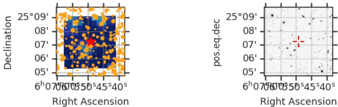
Fig 7. The locations of nearby GAIA DR2 stars with a magnitude difference less than 5 (orange circle) within the Tess Cut Out around TIC 720667477 (red star). Only shown for one sector. Right: SDSS image of the surrounding field.
