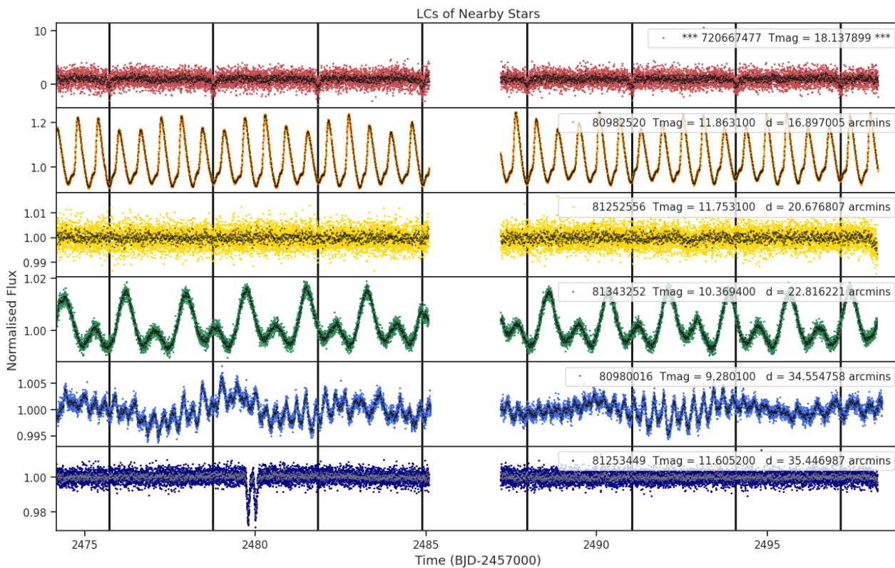
Fig 8. Lightcurves of the five closest stars to target 720667477 (top panel). The distances to the target star and the TESS magnitudes are shown for each star. Only ever shown for one sector.
