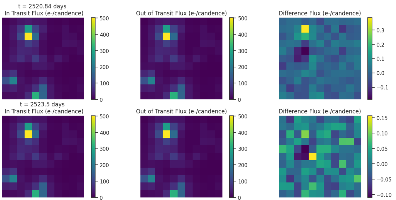
Fig 6. Difference images for target TIC 6553831 for each transit like event. Left: mean in-transit flux(left). Middle: mean out-of-transit flux. Right: difference between the mean out-of-transit and mean in-transit flux. Ensure that the change in brightness occurs on target.
