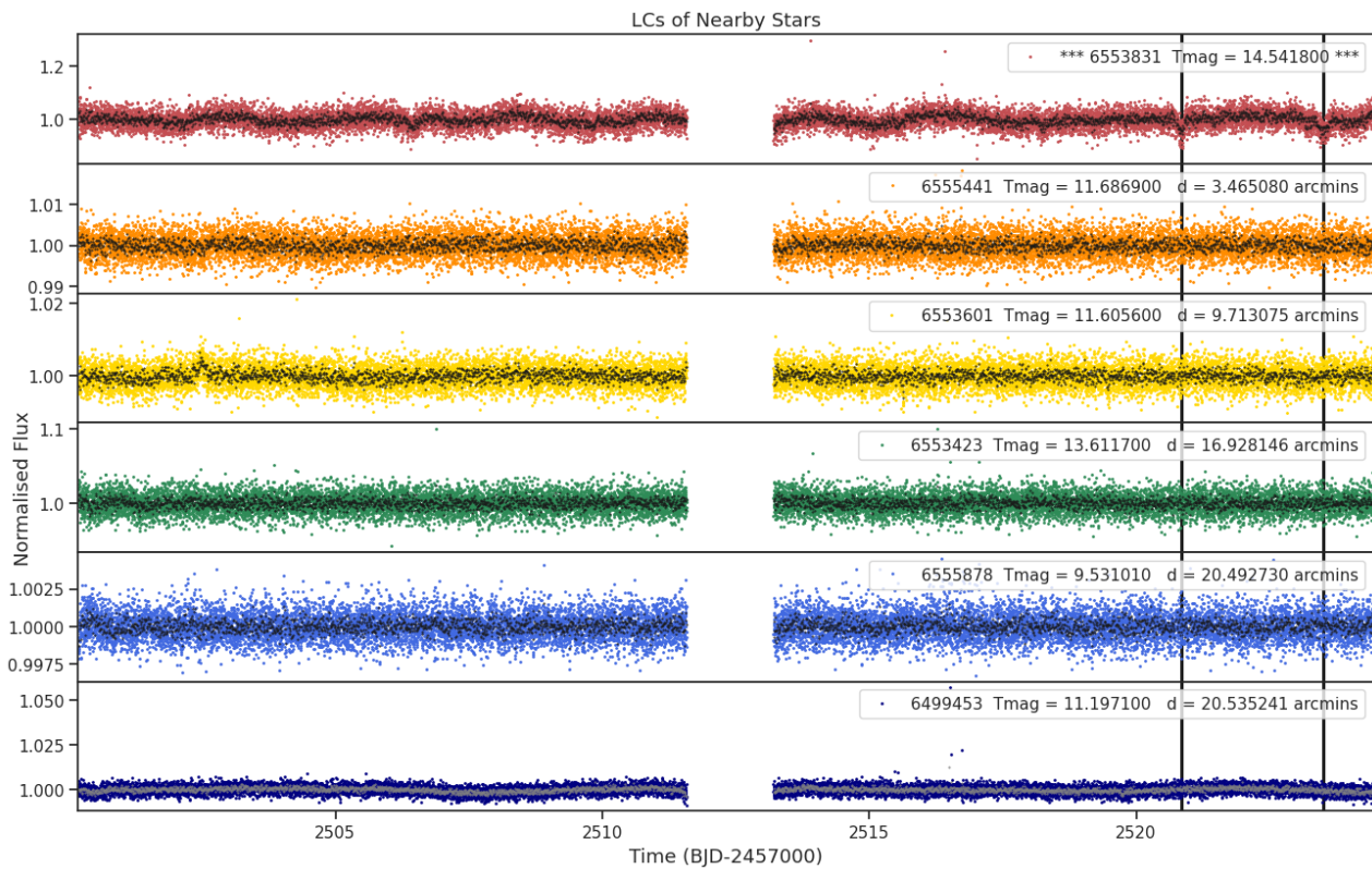
Fig 8. Lightcurves of the five closest stars to target 6553831 (top pannel). The distances to the target star and the TESS magnitudes are shown for each star. Only ever shown for one sector.
