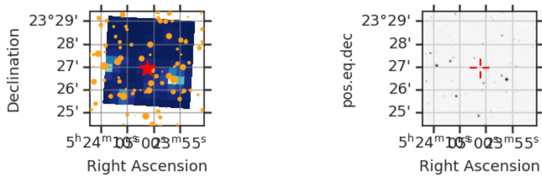
Fig 7. The locations of nearby GAIA DR2 stars with a magnitude difference less than 5 (orange circle) within the TESS Cut Out around TIC 6553831 (red star). Only shown for one sector. Right: SDSS image of the surrounding field.
