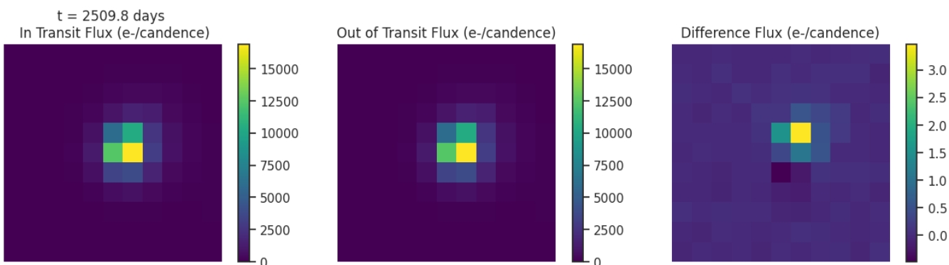
Fig 6. Difference images for target TIC 59490344 for each transit like event. Left: mean in-transit flux(left). Middle: mean out-of-transit flux. Right: difference between the mean out-of-transit and mean in-transit flux. Ensure that the change in brightness occurs on target.
