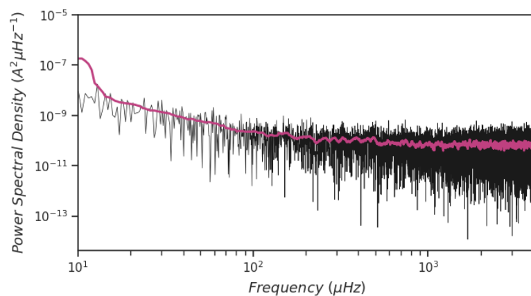
Fig 10. Lomb scargle power spectrum of the TESS lightcurve (black line) and a boxcar-smoothed periogram (pink line) computed with a window length of 20 micro Hz.
