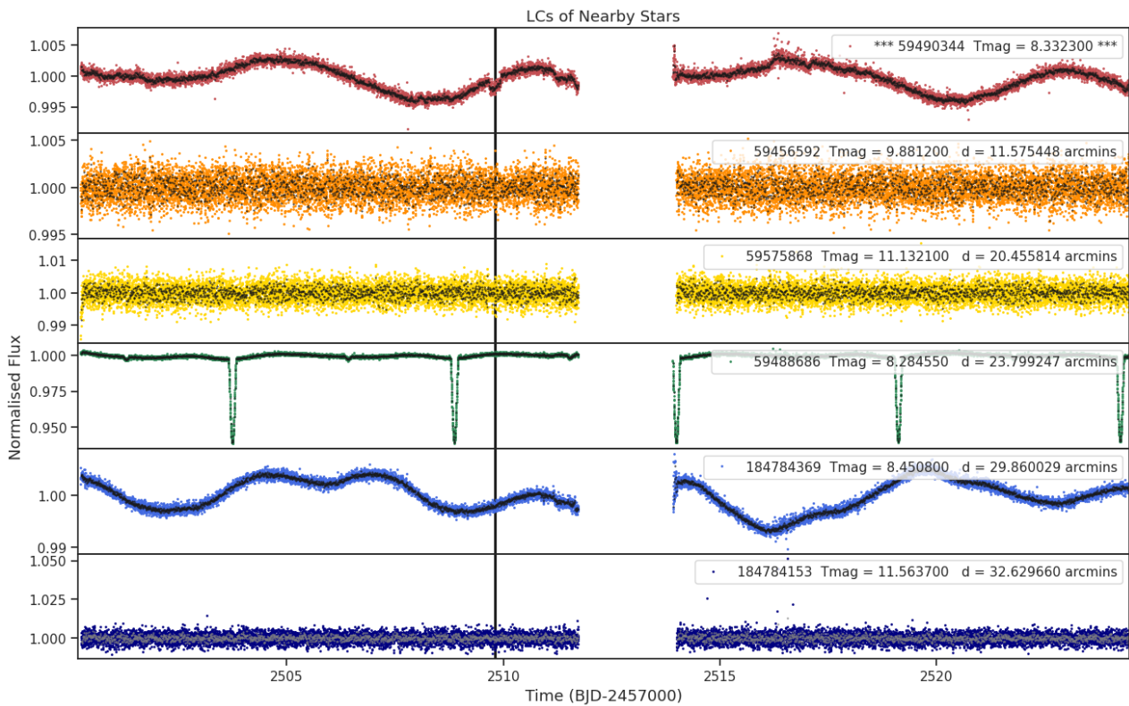
Fig 8. Lightcurves of the five closest stars to target 59490344 (top panel). The distances to the target star and the TESS magnitudes are shown for each star. Only ever shown for one sector.
