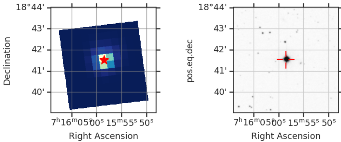
Fig 7. The locations of nearby GAIA DR2 stars with a magnitude difference less than 5 (orange circle) within the TESS Cut Out around TIC 59490344 (red star). Only shown for one sector. Right: SDSS image of the surrounding field.
