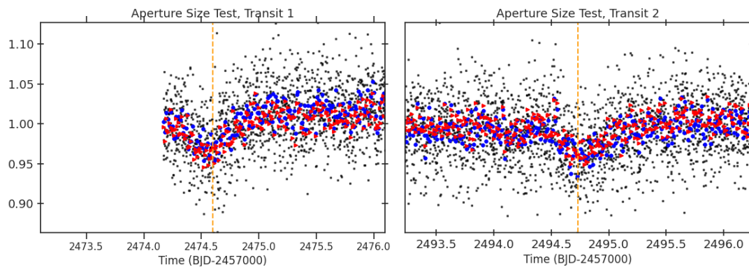
Fig 4. The lightcurve around the time of each transit-like event extracted with the SPOC pipeline defined aperture (binned:blue, uninned:grey) and the with an aperture that is 40 per cent smaller (red). The flux is extracted from the target pixel files (TPFs) and has not been detrended or corrected for systematics. The vertical orange line indicates the time of the transit-like event.
