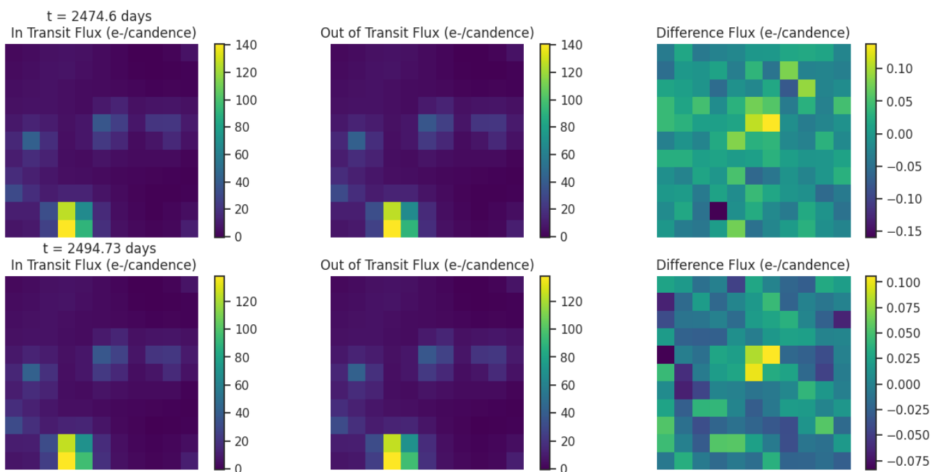
Fig 6. Difference images for target TIC 58175278 for each transit like event. Left: mean in-transit flux(left). Middle: mean out-of-transit flux. Right: difference between the mean out-of-transit and mean in-transit flux. Ensure that the change in brightness occurs on target.
