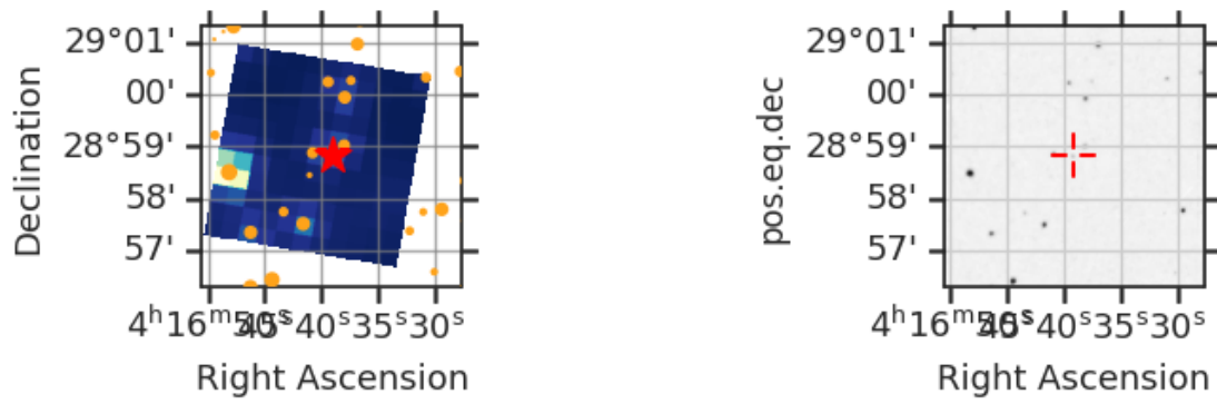
Fig 7. The locations of nearby GAIA DR2 stars with a magnitude difference less than 5 (orange circle) within the TESS Cut Out around TIC 58175278 (red star). Only shown for one sector. Right: SDSS image of the surrounding field.
