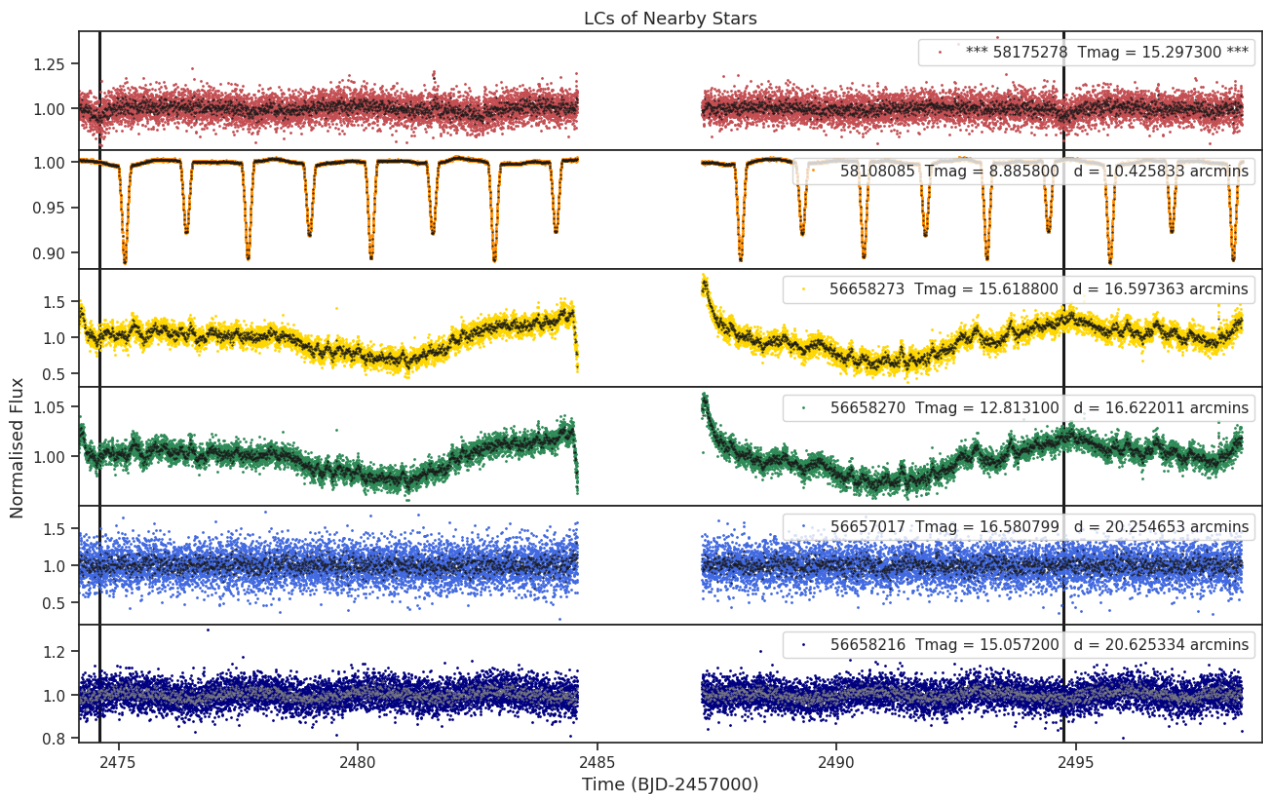
Fig 8. Lightcurves of the five closest stars to target 58175278 (top panel). The distances to the target star and the TESS magnitudes are shown for each star. Only ever shown for one sector.
