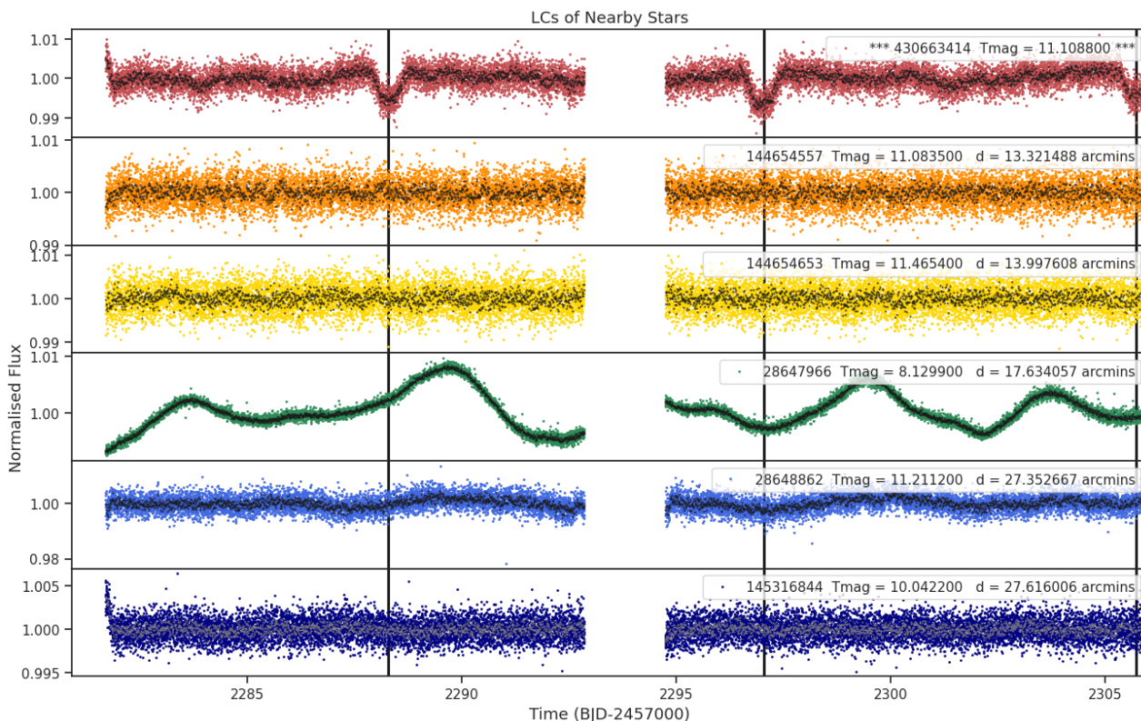
Fig 8. Lightcurves of the five closest stars to target 430663414 (top panel). The distances to the target star and the TESS magnitudes are shown for each star. Only ever shown for one sector.
