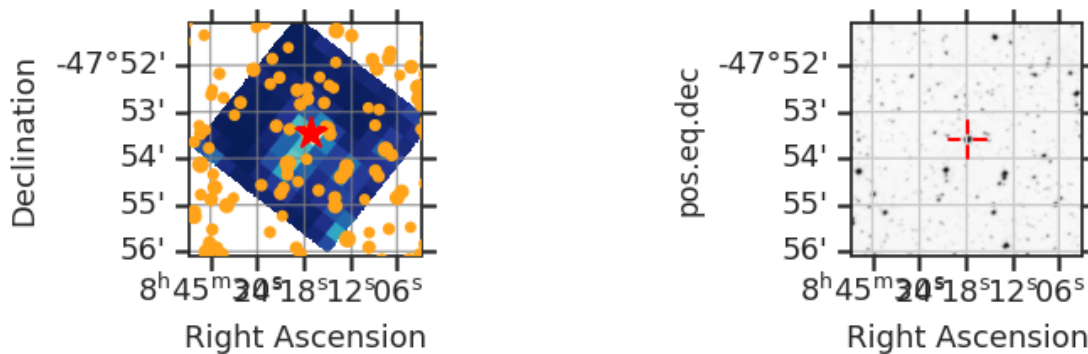
Fig 7. The locations of nearby GAIA DR2 stars with a magnitude difference less than 5 (orange circle) within the Tess Cut Out around TIC 430663414 (red star). Only shown for one sector. Right: SDSS image of the surrounding field.
