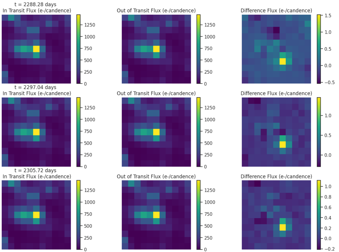
Fig 6. Difference images for target TIC 430663414 for each transit like event. Left: mean in-transit flux(left). Middle: mean out-of-transit flux. Right: difference between the mean out-of-transit and mean in-transit flux. Ensure that the change in brightness occurs on target.
