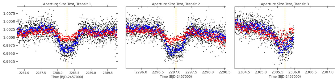
Fig 4. The lightcurve around the time of each transit-like event extracted with the SPOC pipeline defined aperture (binned:blue, unbinned:grey) and the with an aperture that is 40 per cent smaller (red). The flux is extracted from the target pixel files (TPFs) and has not been detrended or corrected for systematics. The vertical orange line indicates the time of the transit-like event.
