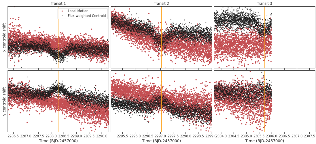
Fig 3. The x and y centroid positions around the time of each transit-like event. The black points shows the CCD column and row position of the target's flux-weighted centroid. The red shows the CCD column and row local motion differential velocity aberration (DVA), pointing drift, and thermal effects. The vertical orange line indicates the time of the transit-like event
