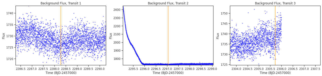
Fig 2. Background flux vs. time around the time of each transit-like event. The vertical orange line indicates the time of the transit-like event.
