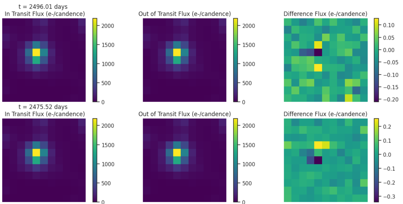
Fig 6. Difference images for target TIC 408195428 for each transit like event. Left: mean in-transit flux(left). Middle: mean out-of-transit flux. Right: difference between the mean out-of-transit and mean in-transit flux. Ensure that the change in brightness occurs on target.
