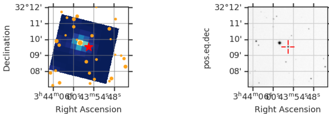
Fig 7. The locations of nearby GAIA DR2 stars with a magnitude difference less than 5 (orange circle) within the Tess Cut Out around TIC 408195428 (red star). Only shown for one sector. Right: SDSS image of the surrounding field.
