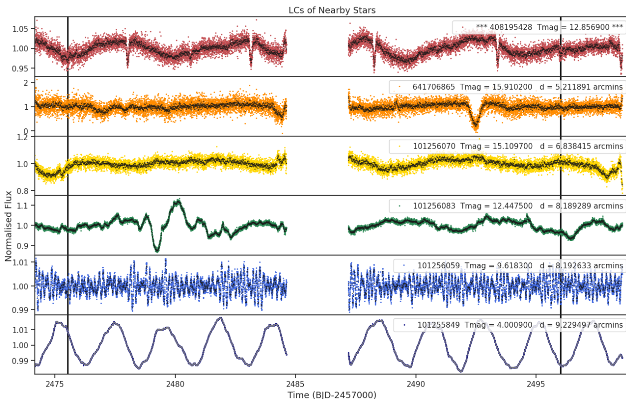
Fig 8. Lightcurves of the five closest stars to target 408195428 (top pannel). The distances to the target star and the TESS magnitudes are shown for each star. Only ever shown for one sector.
