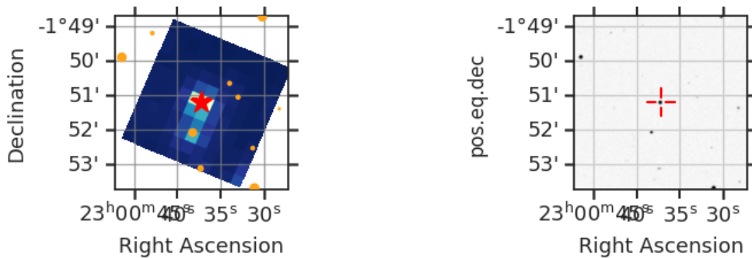
Fig 7. The locations of nearby GAIA DR2 stars with a magnitude difference less than 5 (orange circle) within the Tess Cut Out around TIC 311055966 (red star). Only shown for one sector. Right: SDSS image of the surrounding field.
