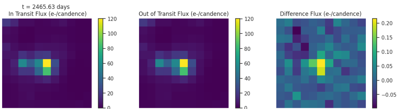
Fig 6. Difference images for target TIC 311055966 for each transit like event. Left: mean in-transit flux(left). Middle: mean out-of-transit flux. Right: difference between the mean out-of-transit and mean in-transit flux. Ensure that the change in brightness occurs on target.
