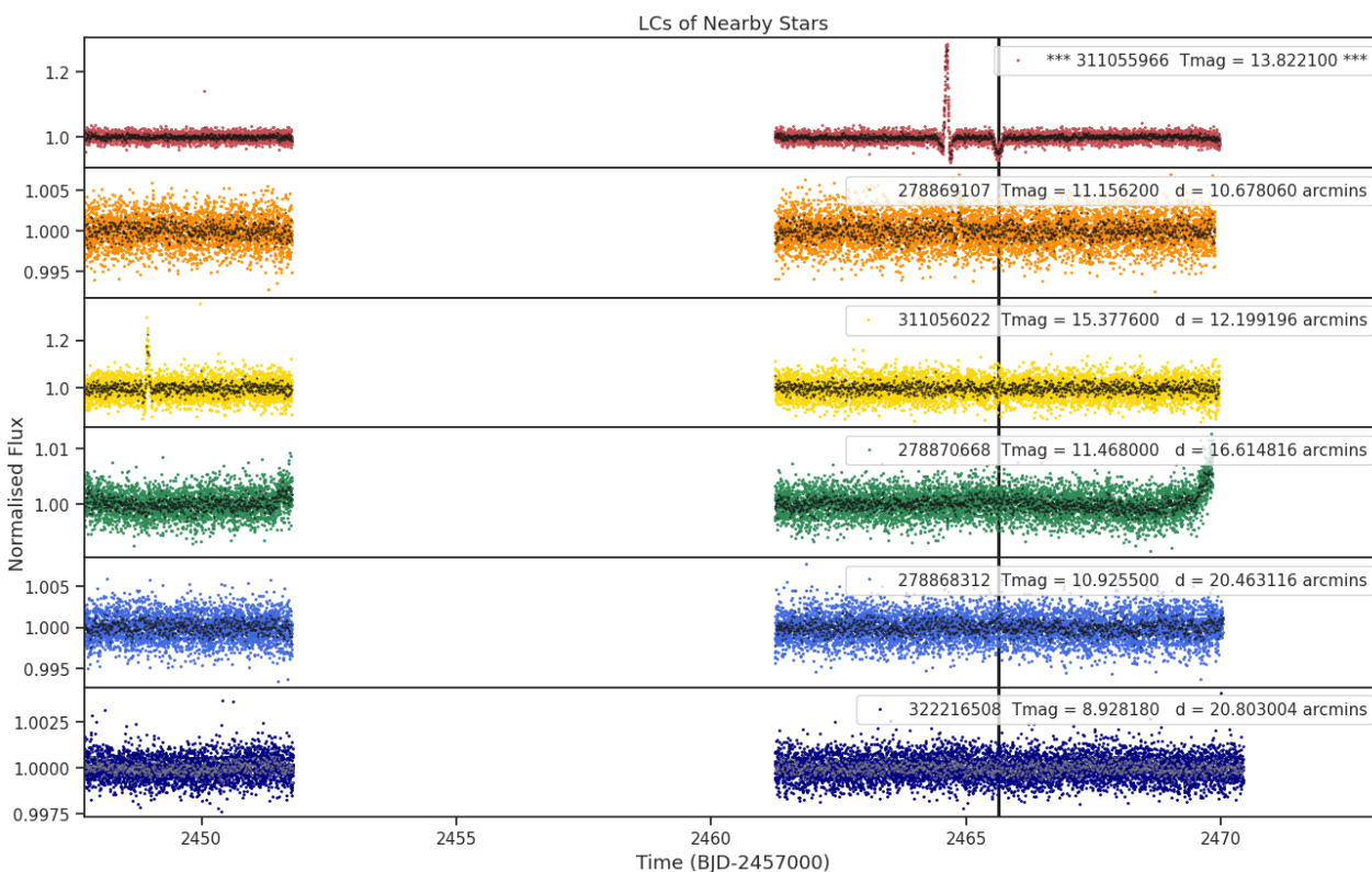
Fig 8. Lightcurves of the five closest stars to target 311055966 (top panel). The distances to the target star and the TESS magnitudes are shown for each star. Only ever shown for one sector.
