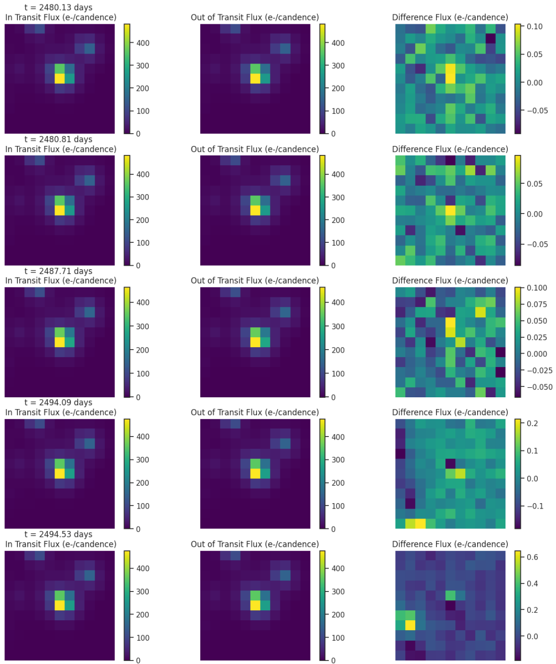
Fig 6. Difference images for target TIC 257395093 for each transit like event. Left: mean in-transit flux(left). Middle: mean out-of-transit flux. Right: difference between the mean out-of-transit and mean in-transit flux. Ensure that the change in brightness occurs on target.
