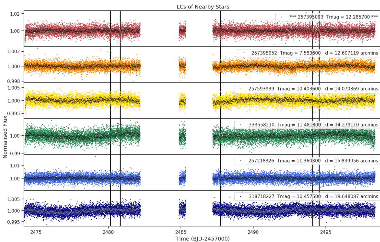
Fig 8. Lightcurves of the five closest stars to target 257395093 (top pannel). The distances to the target star and the TESS magnitudes are shown for each star. Only ever shown for one sector.
