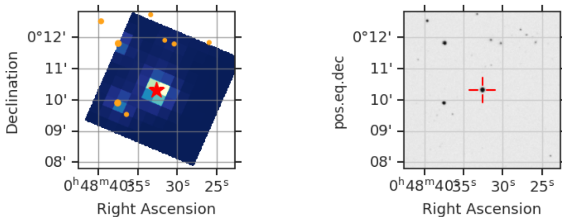
Fig 7. The locations of nearby GAIA DR2 stars with a magnitude difference less than 5 (orange circle) within the Tess Cut Out around TIC 257395093 (red star). Only shown for one sector. Right: SDSS image of the surrounding field.
