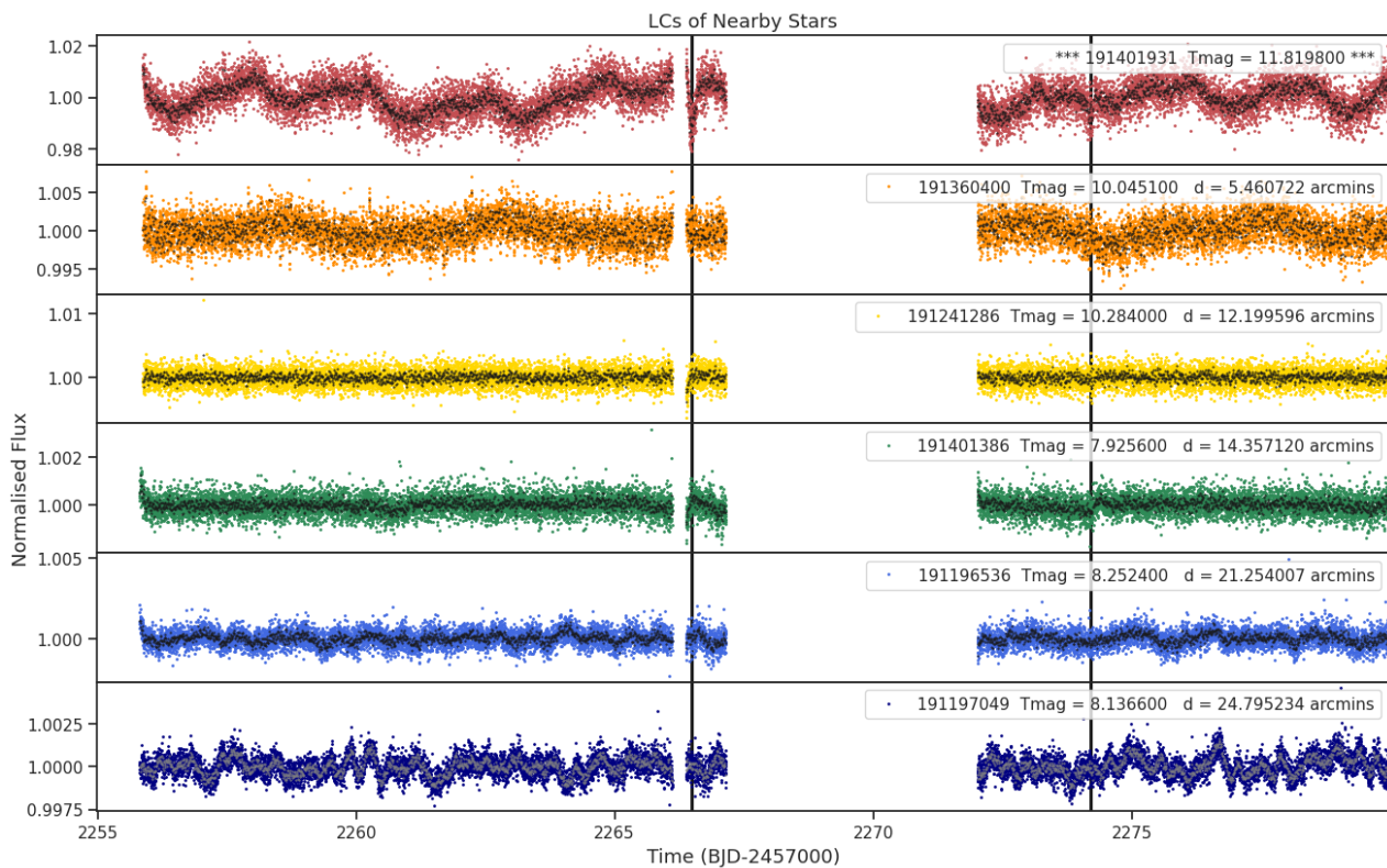
Fig 8. Lightcurves of the five closest stars to target 191401931 (top panel). The distances to the target star and the TESS magnitudes are shown for each star. Only ever shown for one sector.
