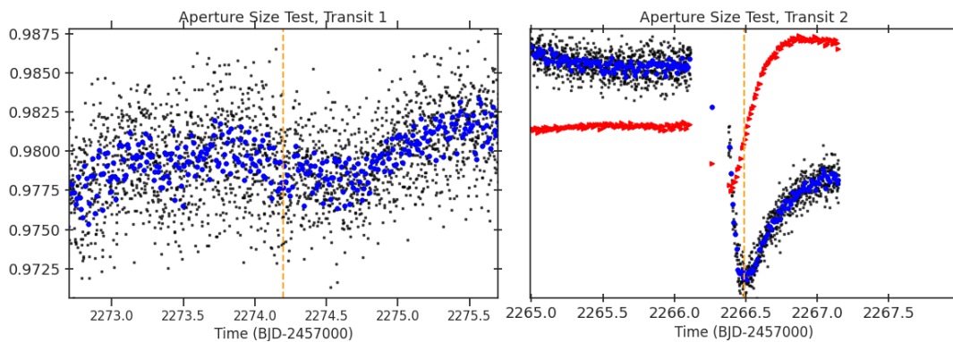
Fig 4. The lightcurve around the time of each transit-like event extracted with the SPOC pipeline defined aperture (binned:blue, unbinned:grey) and the with an aperture that is 40 per cent smaller (red). The flux is extracted from the target pixel files (TPFs) and has not been detrended or corrected for systematics. The vertical orange line indicates the time of the transit-like event.
