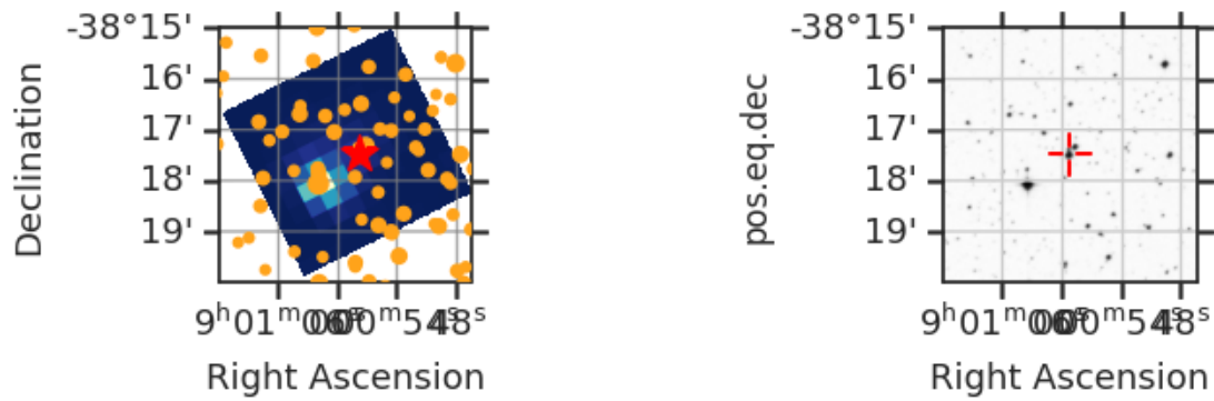
Fig 7. The locations of nearby GAIA DR2 stars with a magnitude difference less than 5 (orange circle) within the TESS Cut Out around TIC 191401931 (red star). Only shown for one sector. Right: SDSS image of the surrounding field.
