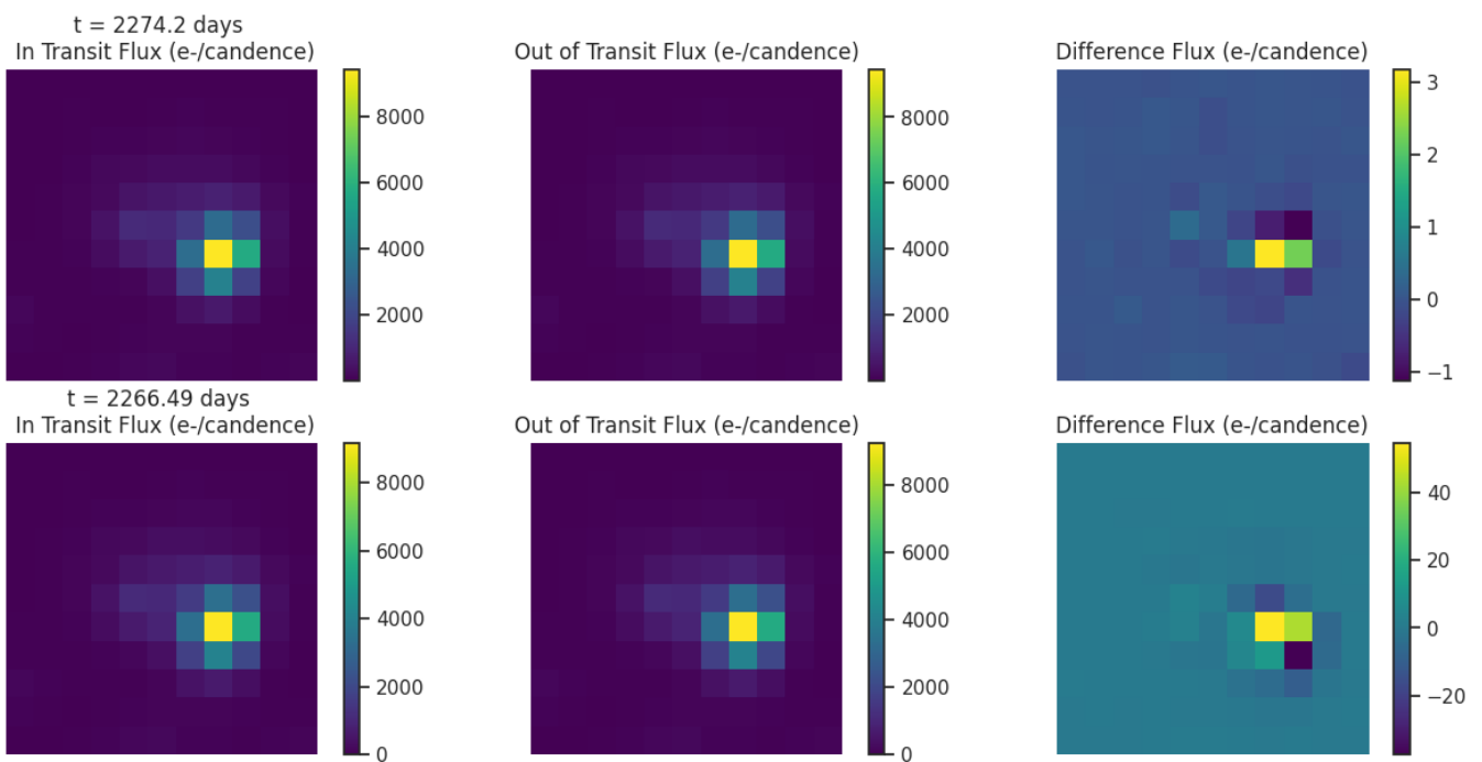
Fig 6. Difference images for target TIC 191401931 for each transit like event. Left: mean in-transit flux(left). Middle: mean out-of-transit flux. Right: difference between the mean out-of-transit and mean in-transit flux. Ensure that the change in brightness occurs on target.
