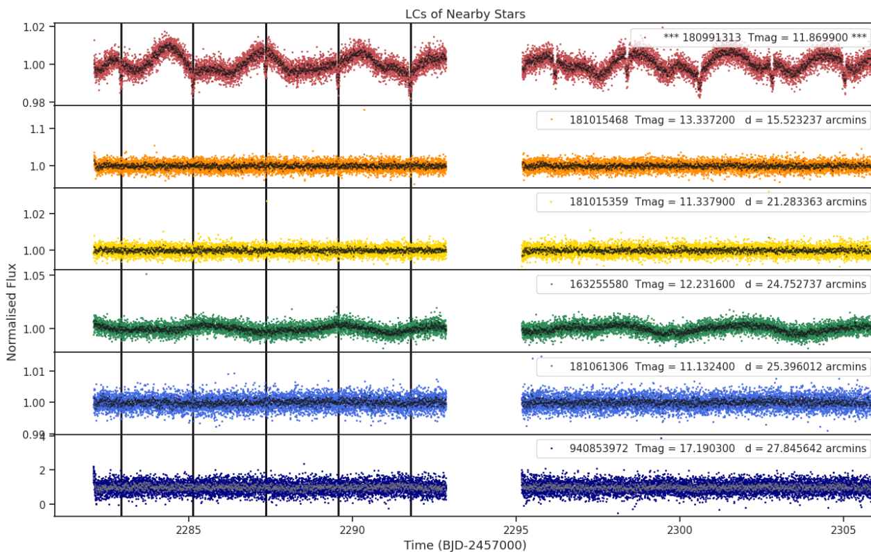
Fig 8. Lightcurves of the five closest stars to target 180991313 (top panel). The distances to the target star and the TESS magnitudes are shown for each star. Only ever shown for one sector.
