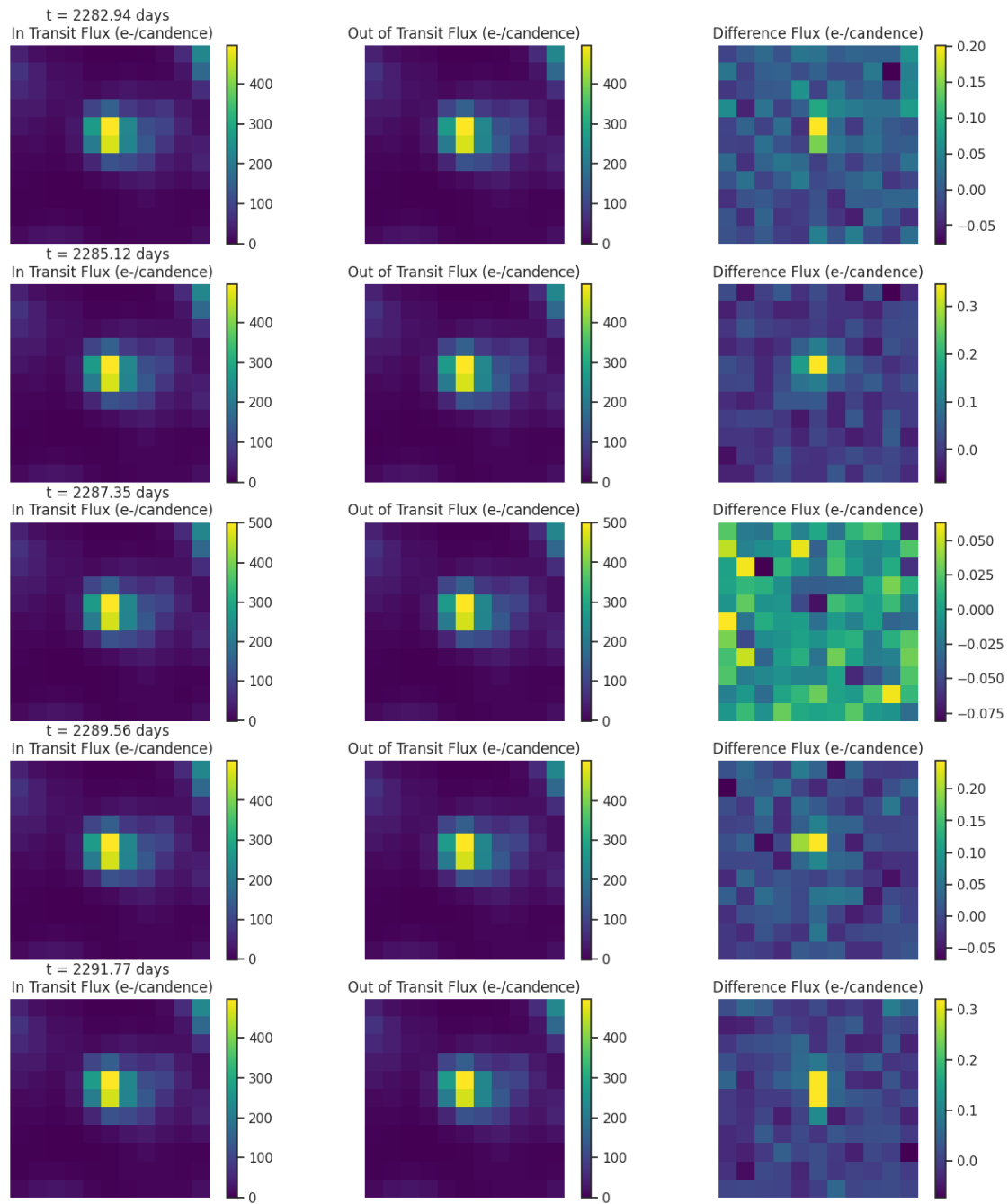
Fig 6. Difference images for target TIC 180991313 for each transit like event. Left: mean in-transit flux(left). Middle: mean out-of-transit flux. Right: difference between the mean out-of-transit and mean in-transit flux. Ensure that the change in brightness occurs on target.
