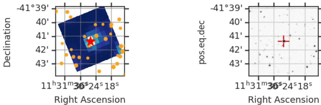
Fig 7. The locations of nearby GAIA DR2 stars with a magnitude difference less than 5 (orange circle) within the Tess Cut Out around TIC 180991313 (red star). Only shown for one sector. Right: SDSS image of the surrounding field.
