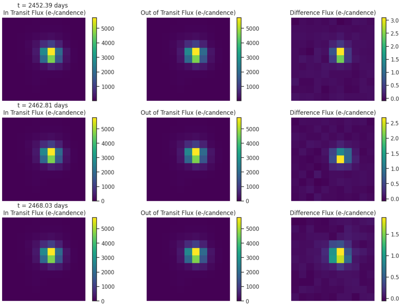
Fig 6. Difference images for target TIC 176220787 for each transit like event. Left: mean in-transit flux(left). Middle: mean out-of-transit flux. Right: difference between the mean out-of-transit and mean in-transit flux. Ensure that the change in brightness occurs on target.
