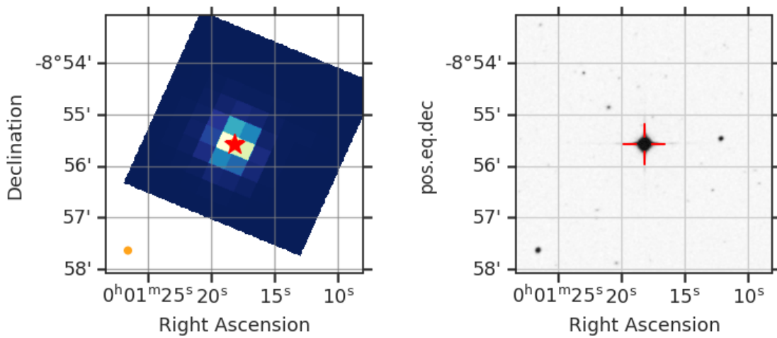
Fig 7. The locations of nearby GAIA DR2 stars with a magnitude difference less than 5 (orange circle) within the TESS Cut Out around TIC 176220787 (red star). Only shown for one sector. Right: SDSS image of the surrounding field.
