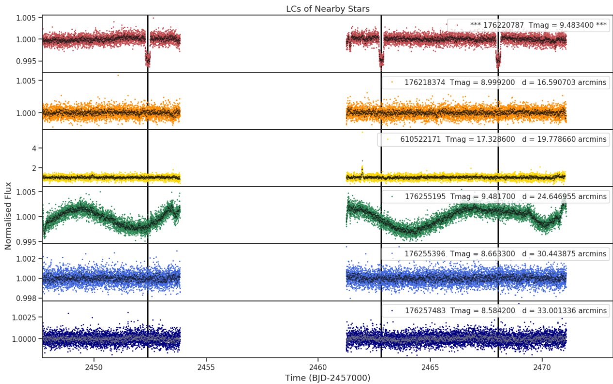
Fig 8. Lightcurves of the five closest stars to target 176220787 (top panel). The distances to the target star and the TESS magnitudes are shown for each star. Only ever shown for one sector.
