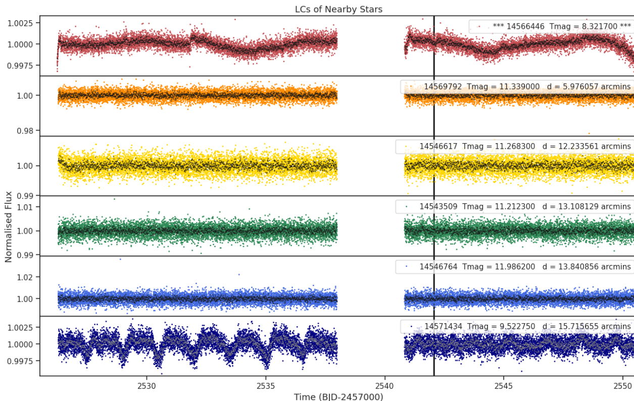
Fig 8. Lightcurves of the five closest stars to target 14566446 (top panel). The distances to the target star and the TESS magnitudes are shown for each star. Only ever shown for one sector.
