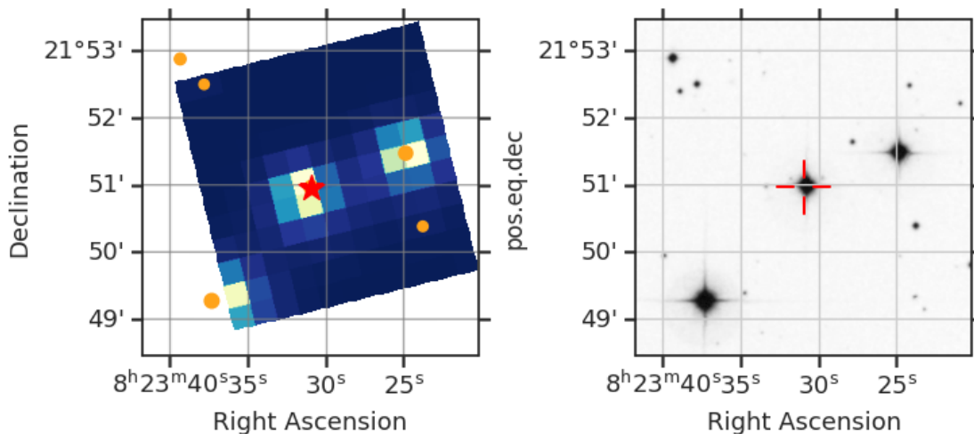
Fig 7. The locations of nearby GAIA DR2 stars with a magnitude difference less than 5 (orange circle) within the TESS Cut Out around TIC 14566446 (red star). Only shown for one sector. Right: SDSS image of the surrounding field.
