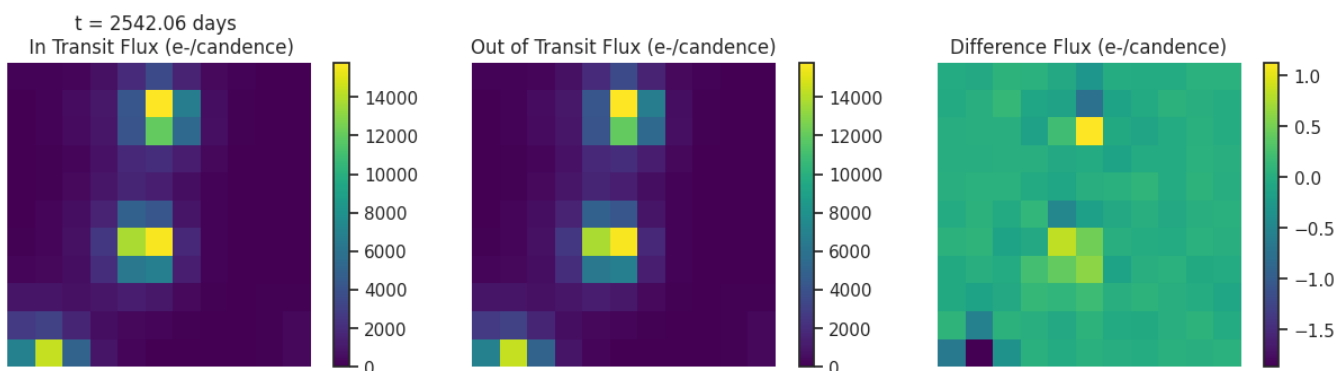
Fig 6. Difference images for target TIC 14566446 for each transit like event. Left: mean in-transit flux(left). Middle: mean out-of-transit flux. Right: difference between the mean out-of-transit and mean in-transit flux. Ensure that the change in brightness occurs on target.
