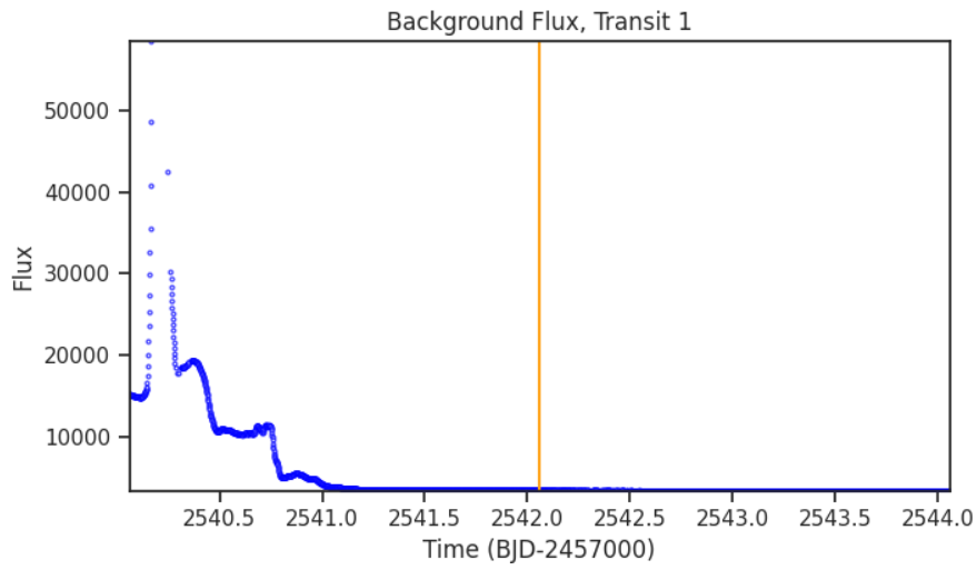
Fig 2. Background flux vs. time around the time of each transit-like event. The vertical orange line indicates the time of the transit-like event.
