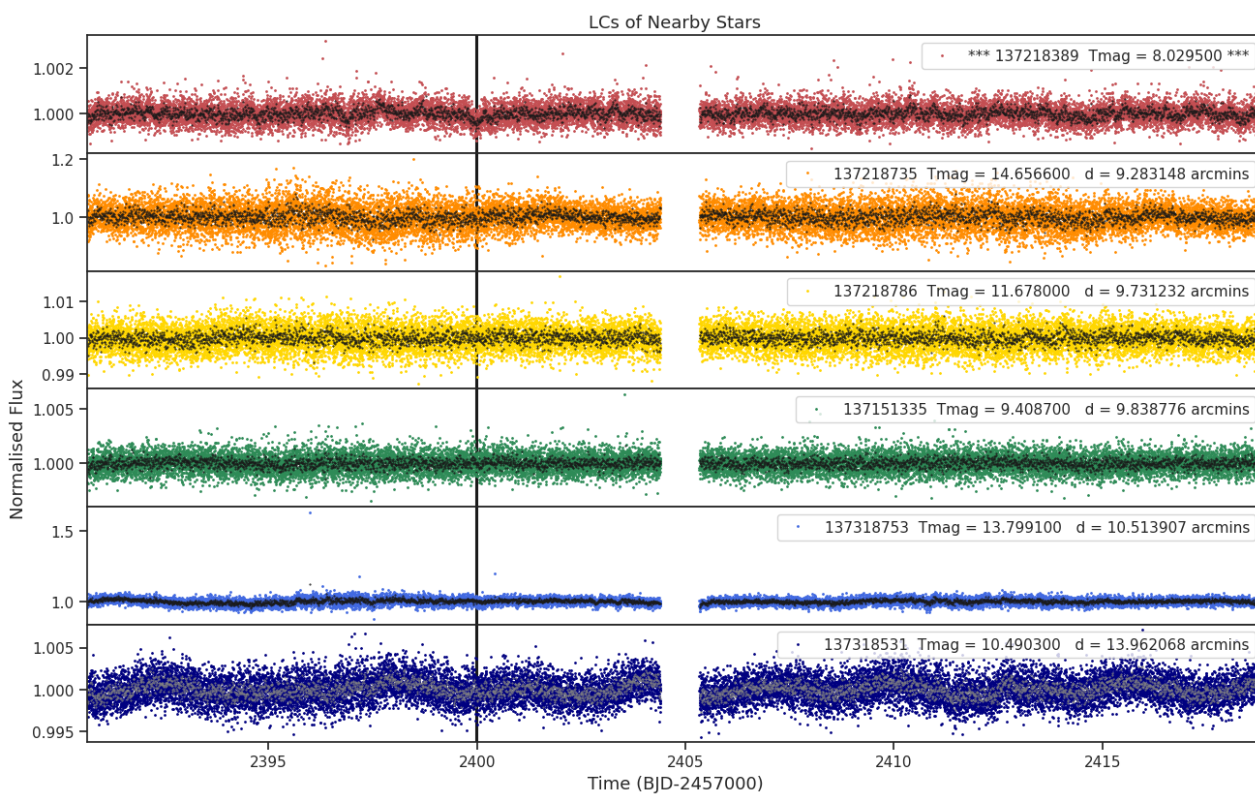
Fig 8. Lightcurves of the five closest stars to target 137218389 (top panel). The distances to the target star and the TESS magnitudes are shown for each star. Only ever shown for one sector.
