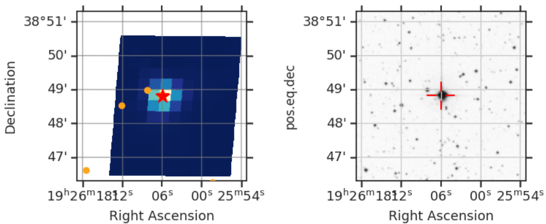
Fig 7. The locations of nearby GAIA DR2 stars with a magnitude difference less than 5 (orange circle) within the Tess Cut Out around TIC 137218389 (red star). Only shown for one sector. Right: SDSS image of the surrounding field.
