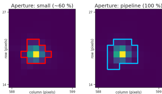
Fig 5. The apertures used to extract the lightcurves. The blue aperture on the right shows the optimum aperture determined by the SPOC pipeline, which is used for the extraction of 2-minute cadence light curves shown in Figure 1. The red outline on the left shows an aperture that is around 40 per cent smaller than the SPOC pipeline aperture which was used to extract the red lightcurve shown in Figure 4.
