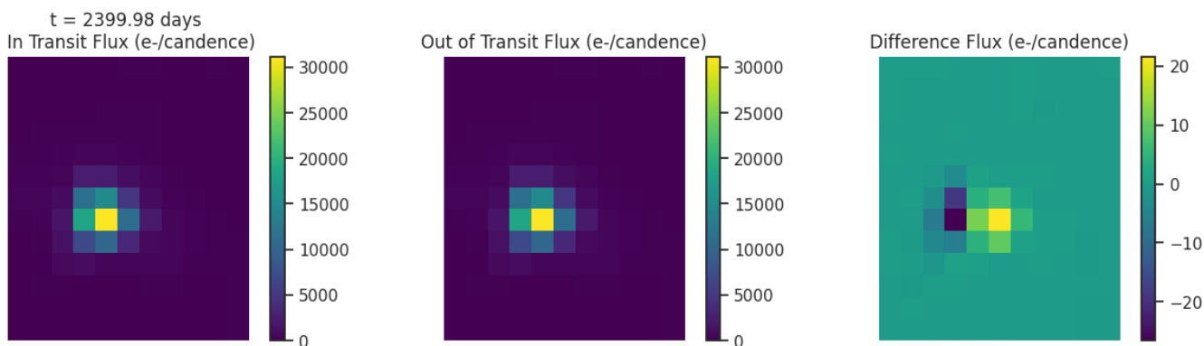
Fig 6. Difference images for target TIC 137218389 for each transit like event. Left: mean in-transit flux(left). Middle: mean out-of-transit flux. Right: difference between the mean out-of-transit and mean in-transit flux. Ensure that the change in brightness occurs on target.
